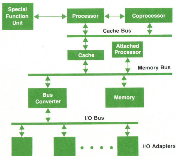
Fig. 3. High-precision architecture system processing unit block diagram, showing high-performance assist processors added to enhance the performance or functionality of the basic system. Special function units connect directly to the processor, and can be thought of as alternative data paths associated with the processor's general registers. Coprocessors, on the other hand, have a control interface with the processor, but they have a private register set and a direct data interface with the cache. They are appropriate when special data types are supported that have little overlap with main processor data types, such as floating-point data. Attached processors are a third level of specialized assist. They have private registers, private data paths, and local storage. Attached processors execute separate instruction streams and are best suited for specialized operations on complex data types—for example, vector processing.
