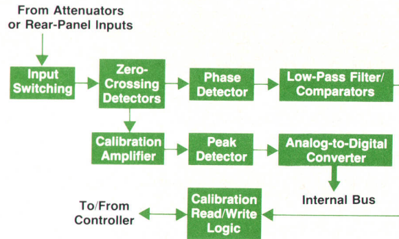
Fig. 2. Phase calibrator basic block diagram.
