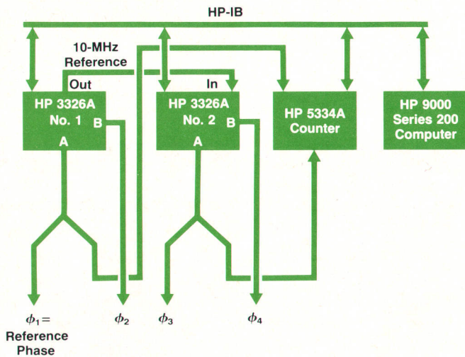
Fig. 2. Connections for four-phase calibration below 1 kHz, showing the additional equipment needed.
