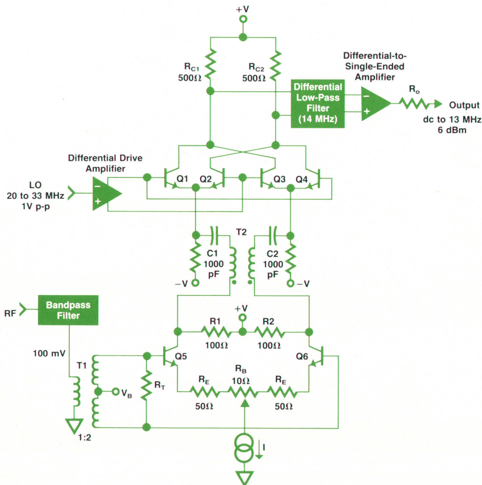
Fig. 6. Simplified schematic diagram of the active mixer in the HP 3326A Two-Channel Synthesizer.
