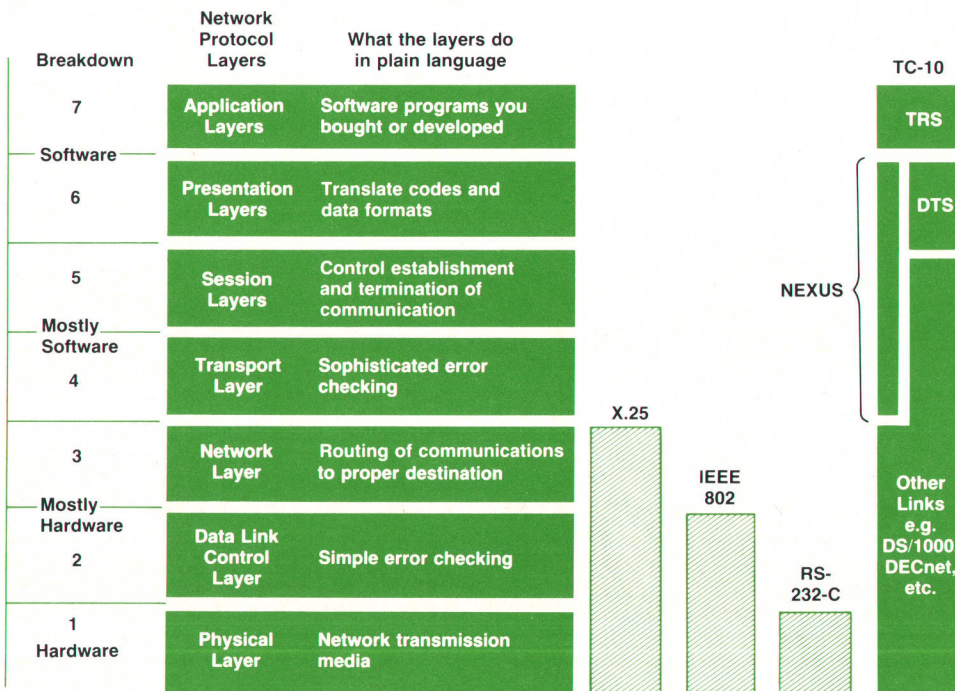
Fig. 3. ISO Open System Interconnect (OSI) model and coverage of TC-10 compared with other network standards.
