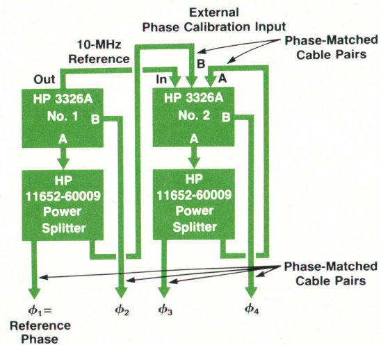
Fig. 1. The HP 3326A Two-Channel Synthesizer can calibrate its phase with respect to any number of other HP 3326As in a minimum number of steps. The normal connections for such multiphase calibration at frequencies above 1 kHz are shown here for four-phase calibration.
