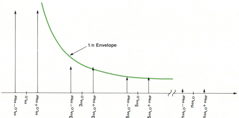
Fig. 3. Spectrum of the mixer IF signal in the ideal case (linear scales).
