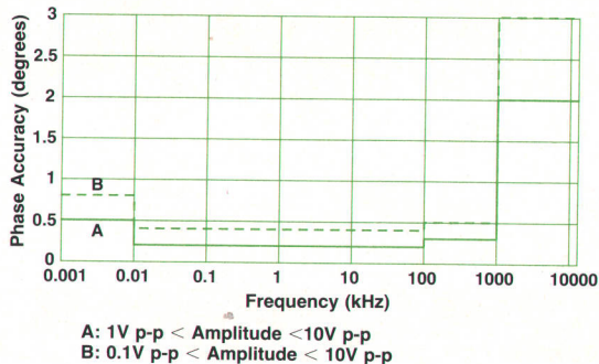
Fig. 1. HP 3326A Two-Channel Synthesizer phase accuracy specifications.
