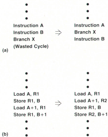
Fig. 2. Branch and load scheduling. (a) One-cycle delayed branches can almost always be used to eliminate a cycle of cache delay by permuting instructions to occupy the branch's "delay slot" usefully. (b) Two ways of moving two words from A, A+1 to B, B+1. The straightforward code on the left incurs "load interlocks" between each load instruction and its adjacent store instruction, since the cache can be expected to require a full cycle to respond. The rescheduled code on the right uses an additional register to overlap the data fetch delays, resulting in a two-cycle saving.
