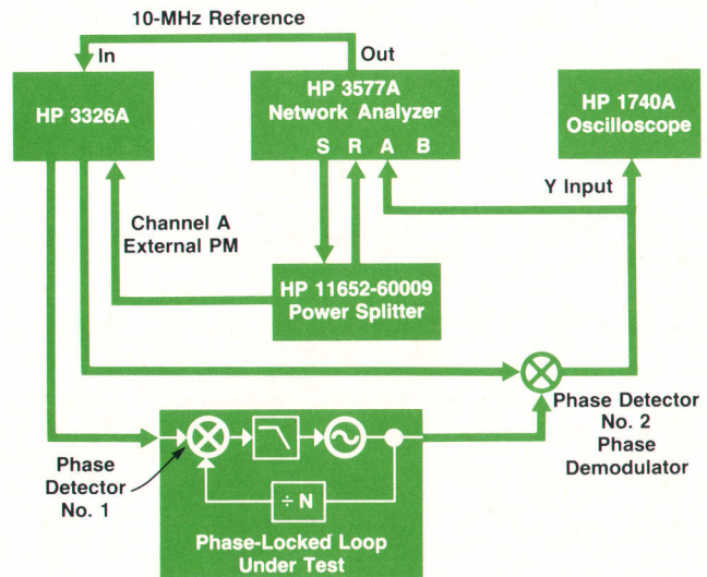
Fig. 3. HP 3326A simplifies the testing of phase-locked loops and control loops. Shown here is a setup for frequency and phase response measurements.
