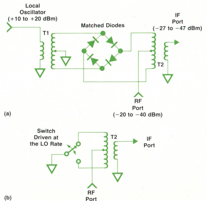
Fig. 2. The classic diode ring mixer (a) and its equivalent circuit (b).
