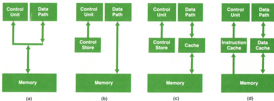
Fig. 1. Computer architecture types: (a) von Neumann (b) microcoded (c) cache (d) proposed.
