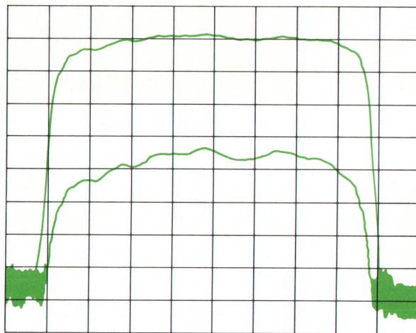
Fig. 3. Swept third-order distortion measurement of an IF amplifier and filter. Distortion level is the difference between the reference trace (upper) and the measurement trace (lower). Vertical scale: 10 dB/division. Horizontal scale: 5 kHz/division.
