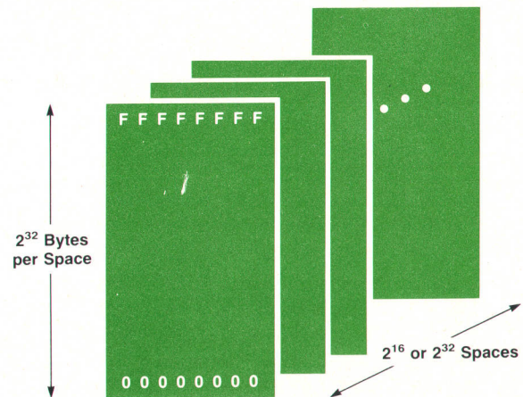
Fig. 1. The new HP architecture provides for up to 2^{32} distinct virtual address spaces, each up to 2^{32} bytes long. Implementations may limit the number of virtual spaces to zero (real addressing only), 2^{16} , or the full 2^{32} .
