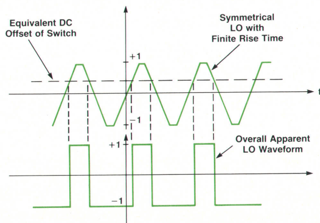
Fig. 5. Effects of LO rise time and system offset on apparent LO symmetry.
