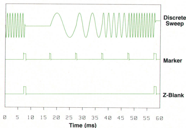
Fig. 1. A discrete sweep with timing signals produced by the HP 3326A Two-Channel Synthesizer.
