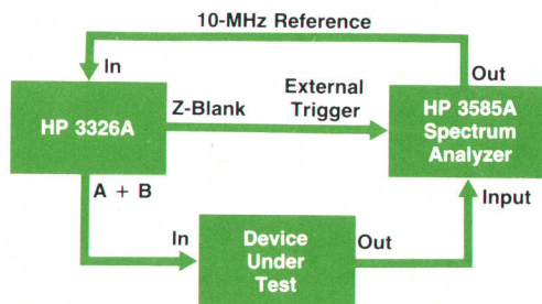
Fig. 2. Setup for swept intermodulation distortion measurements using the HP 3326A Two-Channel Synthesizer.
