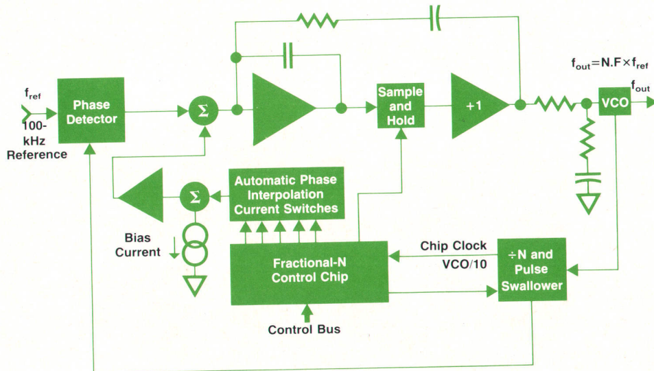
Fig. 5. Fractional-N synthesizer block diagram.
