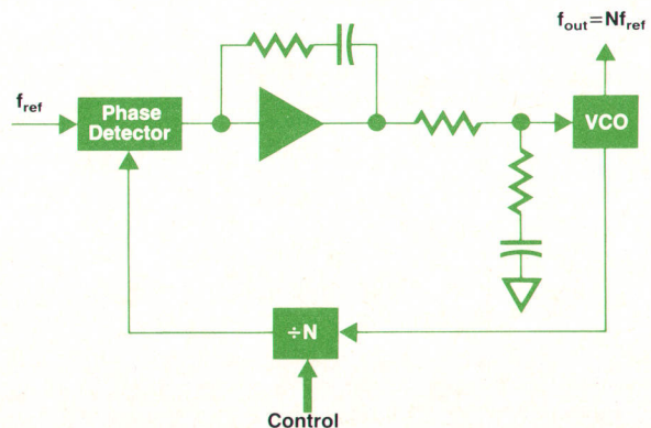
Fig. 4. Conventional \div N phase-locked loop block diagram.
