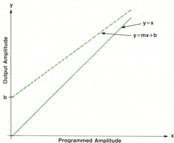
Fig. 2. For an ideal amplitude control system, the output amplitude equals the programmed amplitude (solid line). For a real system, the response (dashed line) differs from the ideal. The HP 3326A firmware measures two points on the actual response curve, computes the slope and intercept, and corrects for system errors.
