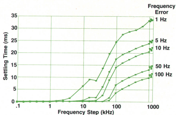
Fig. 2. Typical settling time as a function of the size of the frequency change and allowable frequency error.
