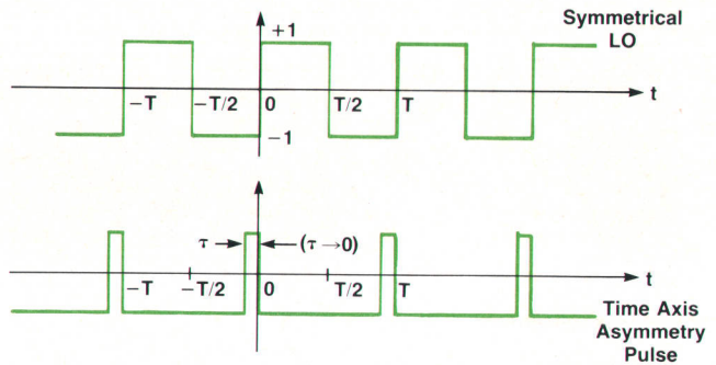
Fig. 4. An asymmetrical LO waveform can be represented as the sum of the square wave and pulse train shown here.
