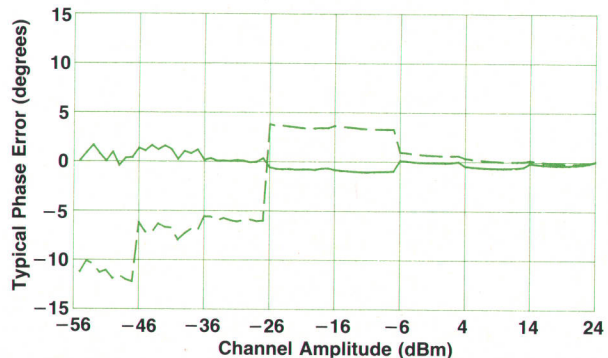
Fig. 3. HP 3326A attenuator phase shift. Dashed line: uncalibrated. Solid line: corrected.
