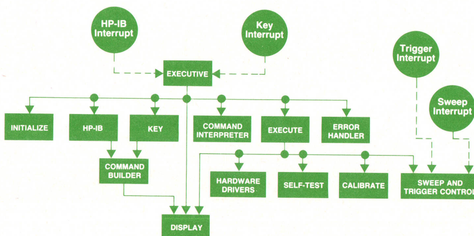
Fig. 1. Firmware architecture of the HP 3326A Two-Channel Synthesizer.
