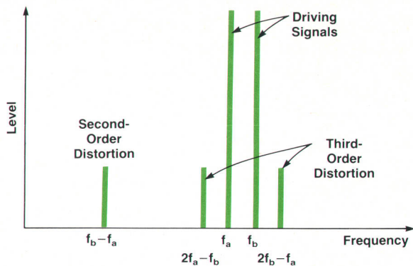
Fig. 1. Second-order and third-order intermodulation distortion products.
