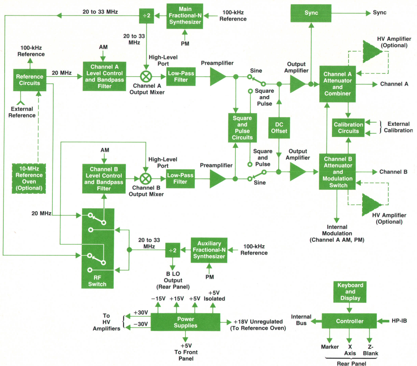
Fig. 2. Simplified HP 3326A block diagram. The functional blocks of a mix-down synthesized signal source appear twice. Fractional-N synthesis provides high-accuracy phase control.
