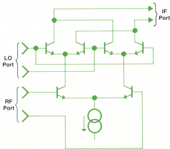
Fig. 1. Basic Gilbert cell multiplier. Bias networks are not shown.
